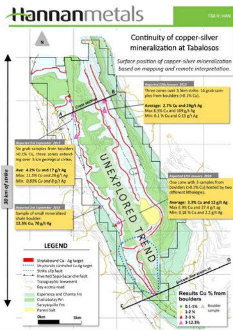
Figure 2. Mapped and inferred stratigraphic position of stratiform copper silver mineralization at Tabalosos based on remote study of detailed topographic terrain corrected elevation data and Sentinel-2 satellite imagery.
